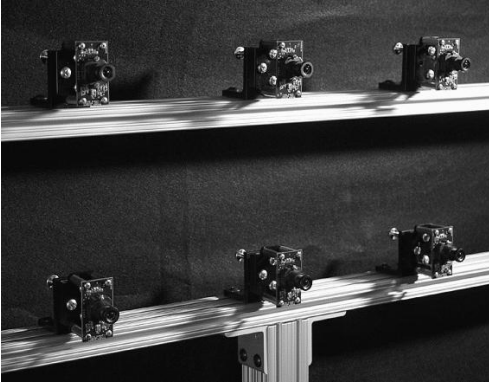
Figure 1: The Stanford Light Field Video Camera consists of numerous CMOS camera heads, arranged in a planar matrix and with aligned optical axes.
