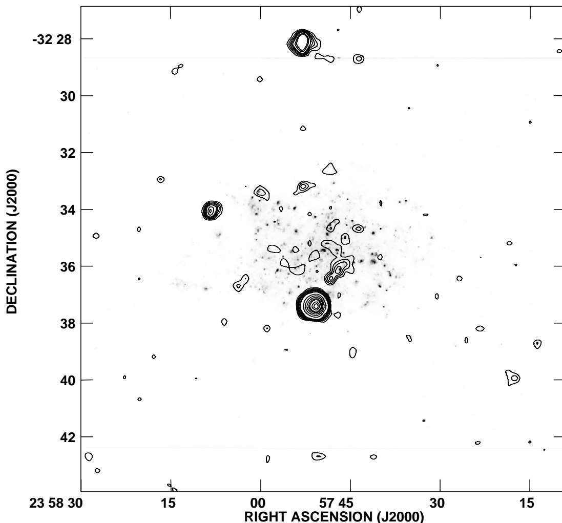
FIG. 1.—X-ray (contours) and H \alpha (gray-scale) image of NGC 7793. The H \alpha image was prepared using observations made with the CTIO, while the X-ray image was prepared using observations made with the ROSAT PSPC instrument over the total energy range of 0.1–2.4 keV with a combined integration of 23,839 s. The noise level in the X-ray image is 9.4 \times 10^{-4} counts \text{arcmin}^{-2} , and the contours are set at the 3 \sigma , 4.5 \sigma , 6 \sigma , 7.5 \sigma , 9 \sigma , 12 \sigma , 14 \sigma , 30 \sigma , 45 \sigma , 60 \sigma , 75 \sigma , 85 \sigma , 105 \sigma , and 120 \sigma level.
