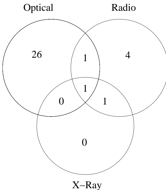
FIG. 9.—Venn diagrams depicting the intersection of selected sets of SNRs (X-ray, optical, and radio) for the galaxies M33, NGC 300, and NGC 7793. The galaxies have been arranged in order of increasing distance. Notice how limited the intersection between the three sets becomes with increasing distance to the galaxy.
